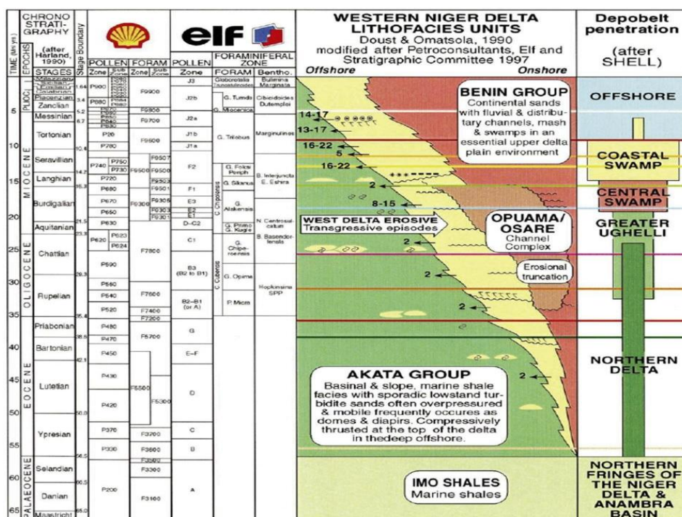
Fig. 2. Regional stratigraphy of Western Niger Delta [15]
