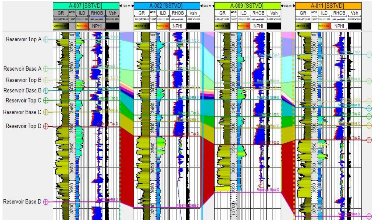
Fig. 8. Shale volume values calculated for the four reservoir intervals and correlated across all four wells
