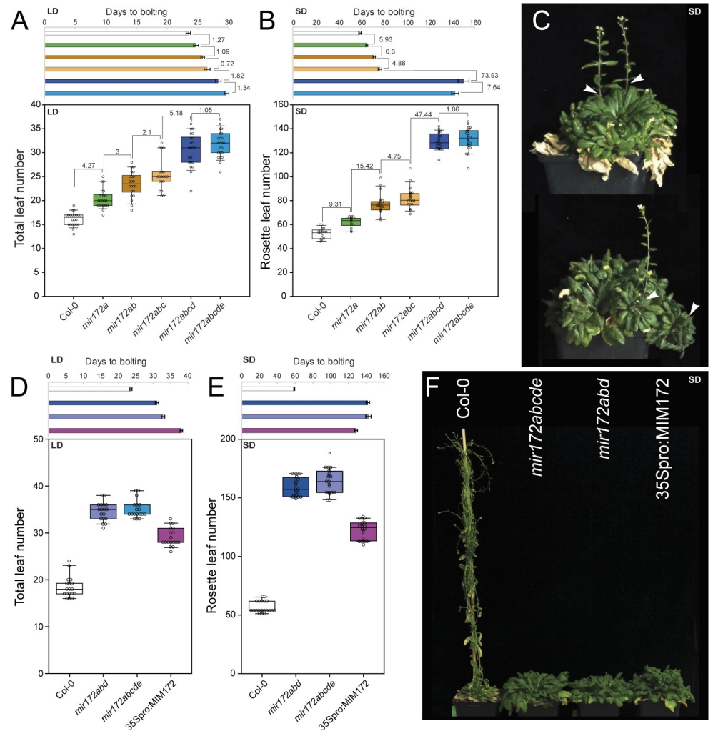
Fig 3. Flowering time of higher-order mir172 mutants in LDs and SDs. (A, B) Graphs depicting DTB and TLN or RLN of Col-0, mir172a-2 , mir172a-2 b-3 , mir172a-2 b-3 c-1 , mir172a-2 b-3 c-1 d-3 , and mir172a-2 b-3 c-1 d-3 e-1 mutant combinations in LD (A) and SD (B) conditions. The difference between the means of the indicated genotypes is shown above the box plots. Data underlying panels (A) and (B) are provided in S2 Data . (C) Photographs of mir172a-2 b-3 c-1 d-3 e-1 plants after approximately 6 months of growth under SD conditions. Plant initiated flowering shoots from axillary meristems (white arrowheads) rather than the primary meristem. (D, E) Graphs depicting DTB and total or RLN of Col-0, mir172a-2 b-3 d-2 , mir172a-2 b-3 c-1 d-3 e-1 mutant combinations and 35Spro:MIM172 in LD (D) and SD (E) conditions. Data underlying panels (D) and (E) are provided in S2 Data . (F) A photograph of Col-0, mir172a-2 b-3 d-2 , mir172a-2 b-3 c-1 d-3 e-1 mutant combinations and 35Spro:MIM172 grown under SD conditions. DTB, days to bolting; LD, long-day; RLN, Rosette leaf number; SD, short-day; TLN, total leaf number.
