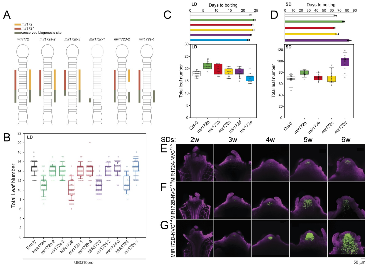
Fig 2. Functional analysis of single mir172 mutants LDs and SDs. (A) Schematic depicting the structure of a representative “reference” miR172 precursor and the mutant forms generated using CRISPR-Cas-9 DNA editing. The orange, red, and green bars represent the coding sequences for miR172, miR172*, and the biogenesis site required for DCL1 cleavage, respectively. Truncation of these bars and opaque sections of the mutant miR172 precursor indicates the regions that were deleted via CRISPR-Cas-9 in mir172a-2 , mir172b-3 , mir172c-1 , mir172d-2 , and mir172e-1 . (B) A graph depicting the TLN of first generation transformants in a Col-0 background harboring a T-DNA containing only the UBQ10pro-3’OCS promoter-terminator cassette or expressing reference Col-0 or mutated versions of the indicated MIR172 gene under the control of the UBQ10pro-3’OCS cassette. (C, D) Graphs depicting the TLN and bolting times of WT and plants harboring single mir172 mutations in (C) LD and (D) SD conditions. Data underlying panels B–D are provided in S2 Data. (E–G) Confocal laser scanning micrographs of the shoot apices of (E) MIR172A-NVG, (F) MIR172B-NVG, and (G) MIR172D-NVG transgenic plants grown in SD conditions and harvested at the indicated times after germination. Fluorescence from the Venus protein is artificially colored in green, and the fluorescence from the Renaissance dye is artificially colored in magenta. Cas-9, CRISPR associated protein-9; CRISPR, clustered regularly interspaced short palindromic repeats; LD, long-day; NVG, NLS-Venus-GUS; SD, short-day; TLN, total leaf number; WT, wild-type.
