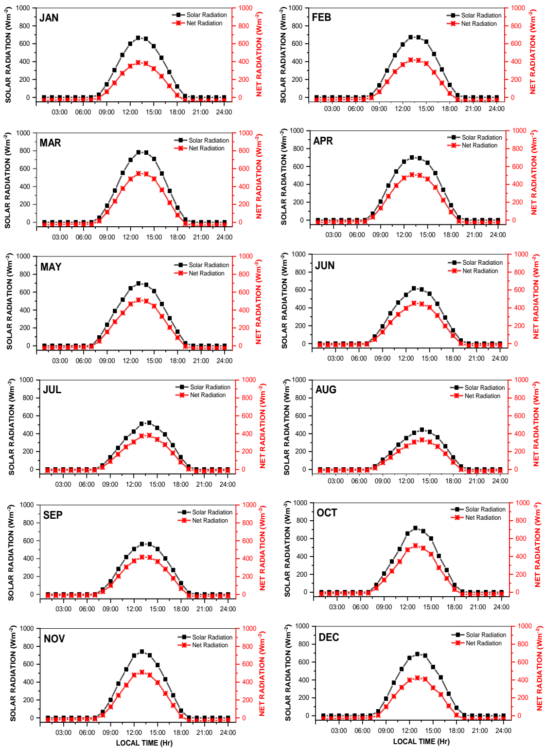
Fig. 1. Diurnal variations of monthly mean solar radiation and net radiation
