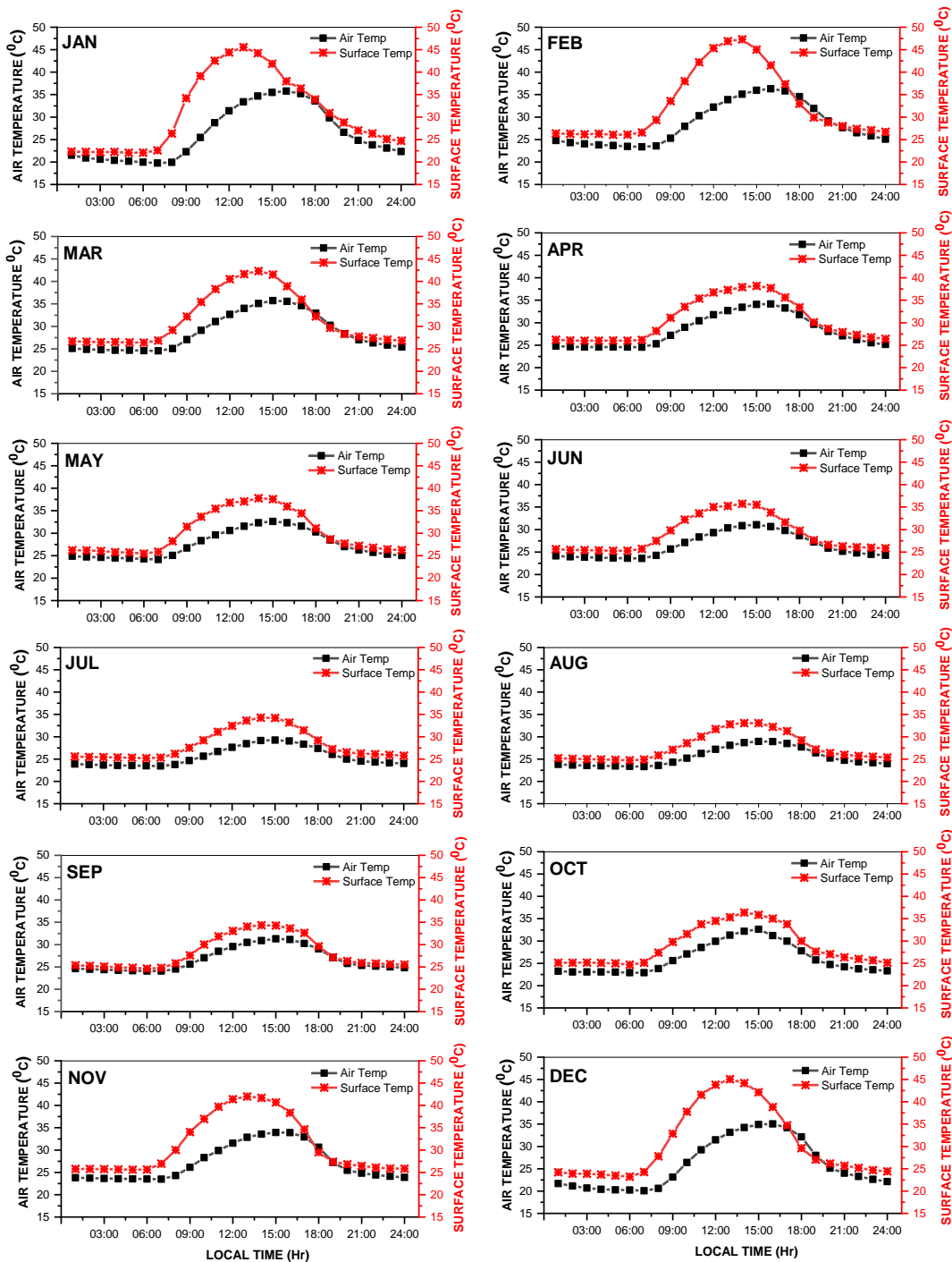
Fig. 2. Diurnal variations of monthly mean air temperature and surface temperature
