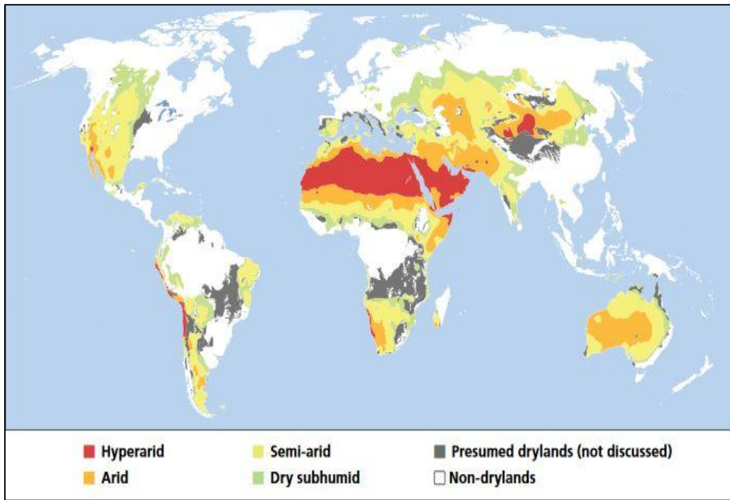
Fig. 1. Global distribution of the arid and semi-arid regions [4]
