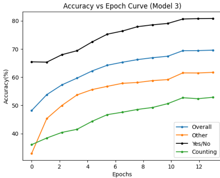
Fig. 21. Accuracy vs epoch curve (Model 3)
