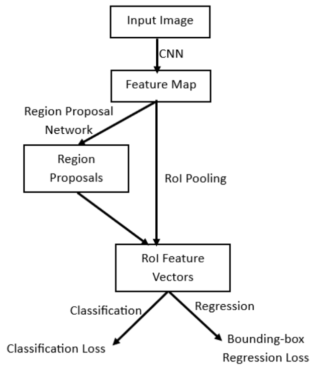
Fig. 6. Faster RCNN flow diagram
