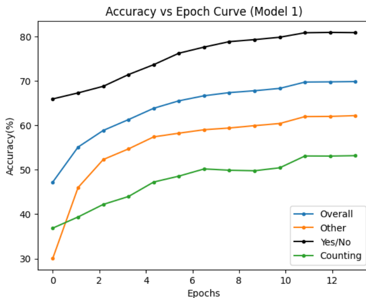
Fig. 19. Accuracy vs epoch curve (Model 1)
