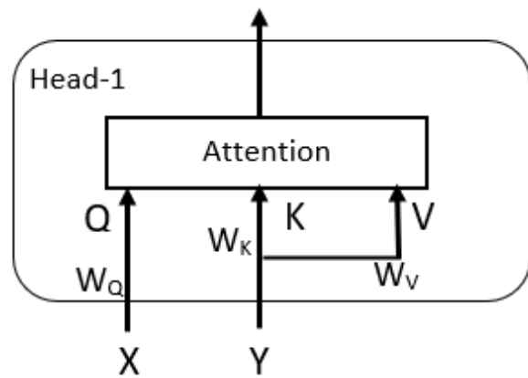
Fig. 10. Guided-attention
