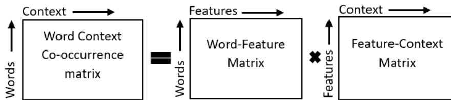
Fig. 7. GloVe matrix decomposition
