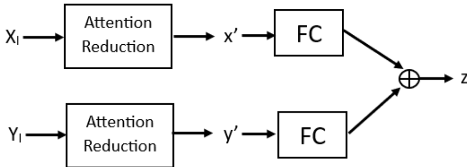
Fig. 11. Features fusion
