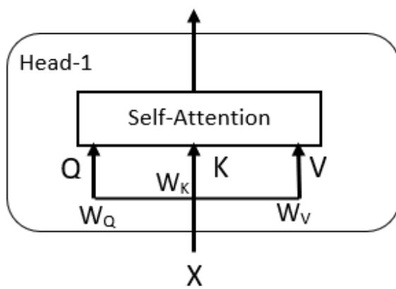
Fig. 9. Self-attention
