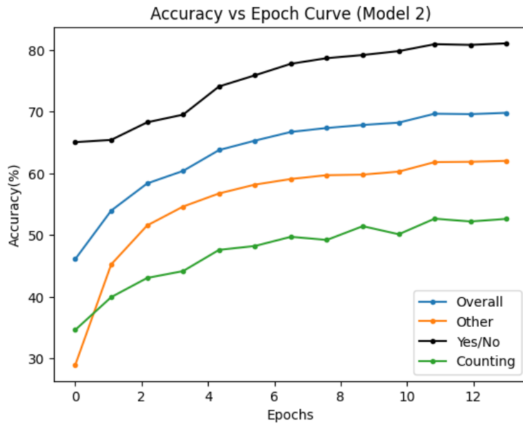
Fig. 20. Accuracy vs epoch curve (Model 2)
