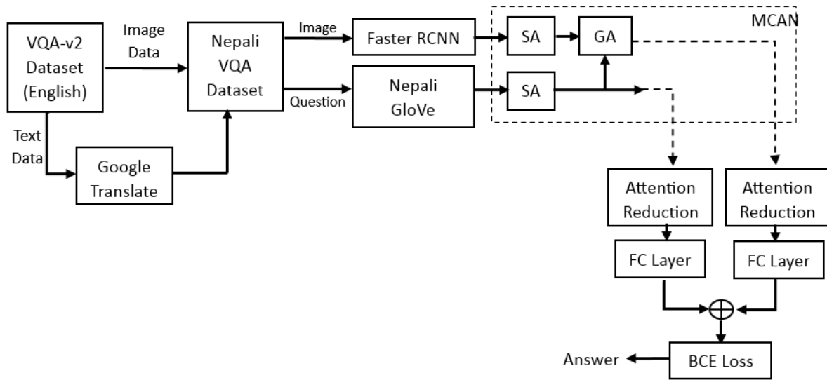
Fig. 12. Overall working principle
