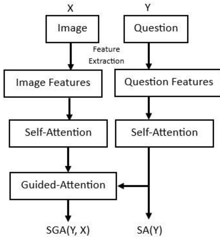
Fig. 8. MCA flow diagram
