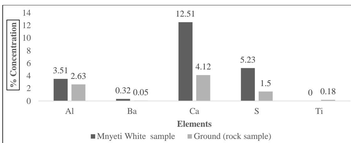
Fig. 4. Comparison of concentration of elements in white pigment and ground (rock sample) from the Mnyeti site
