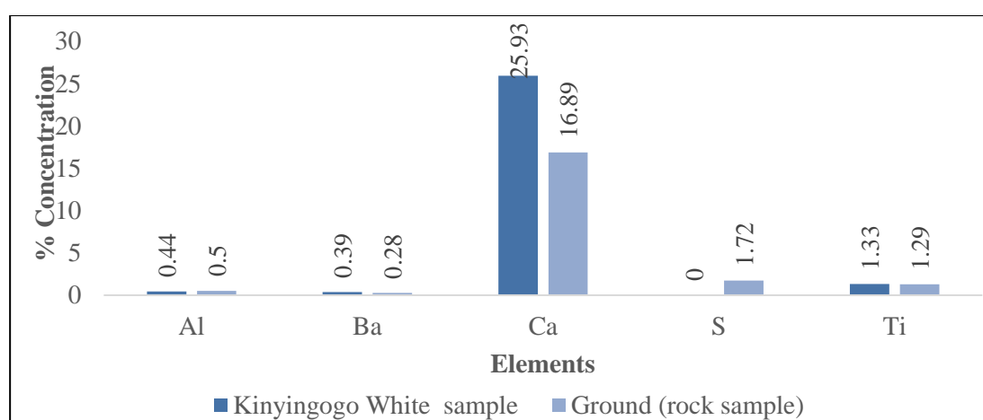
Fig. 5. Comparison of concentration of elements in white pigment and rock sample from Kinyingogo site
