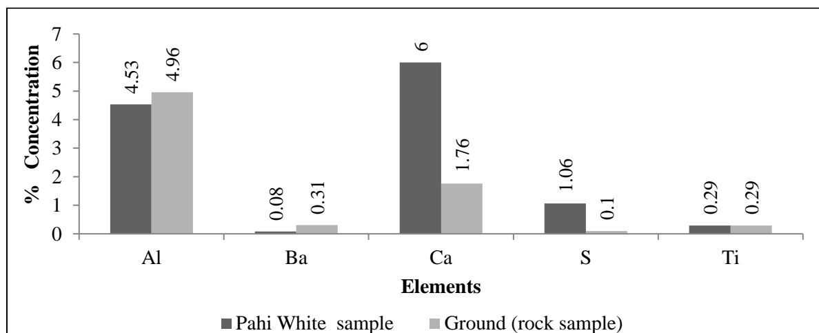
Fig. 2. Comparison of concentration of elements in white pigment and ground (rock sample) from Pahi site
