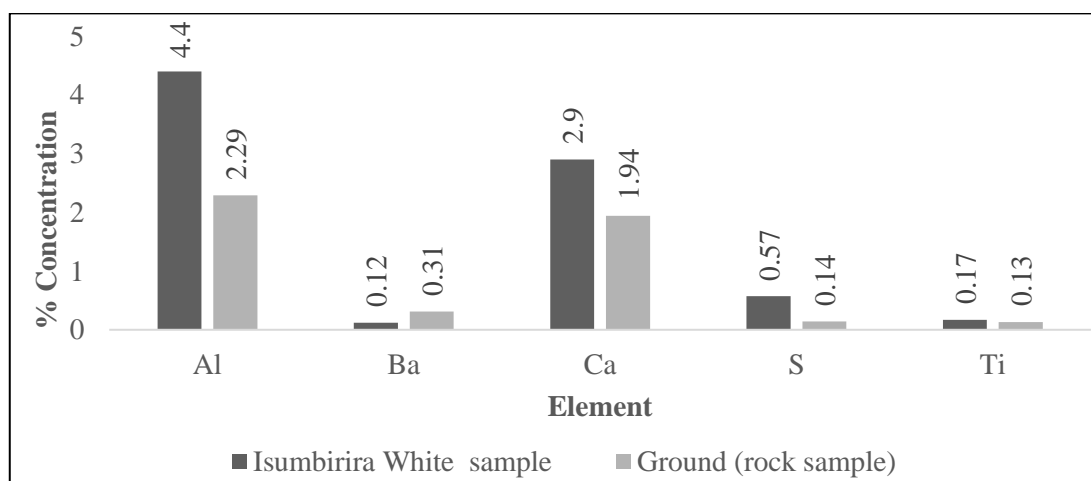
Fig. 3. Comparison of concentration of elements in white pigment and rock sample from the Isumbirira site
