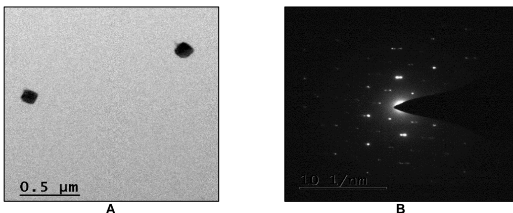
Fig. 4. TEM photomicrograph (A) and SAED (B) of optimized LCZ – LPG
