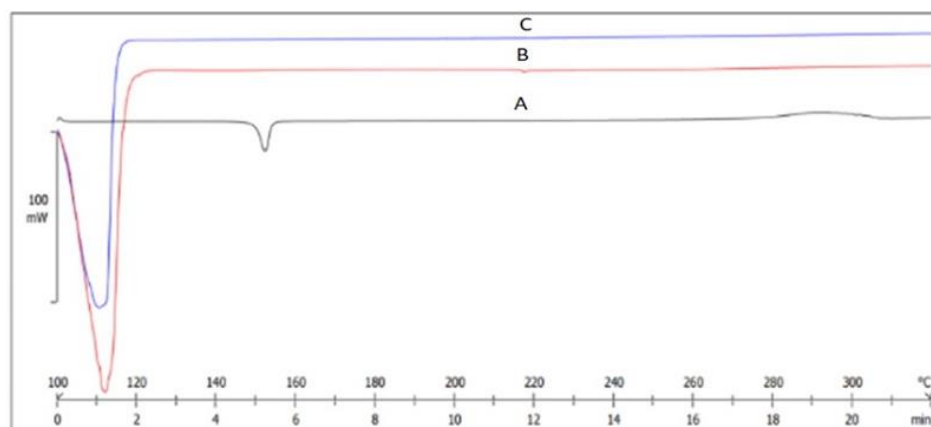
Fig. 3. DSC thermograms of pure drug (A), Blank leciplex (B) and LCZ-LP (C)
