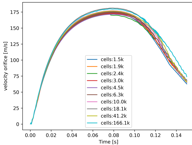
Figure 3. Grid independence study showing convergence of pressure (top) and velocity (bottom) at the orifice.
