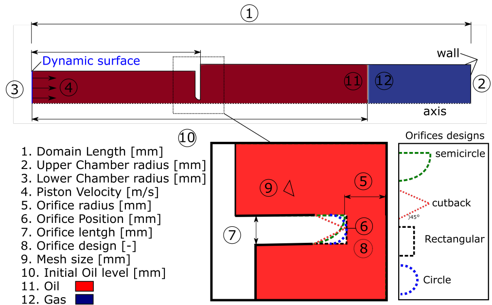
Figure 1. Geometry schematic of shock absorber.
