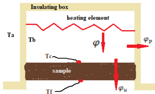
Fig. 3. Sample in thermal box
