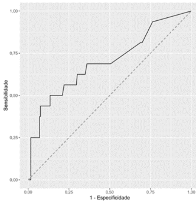
Fig. 2. ROC Curve
