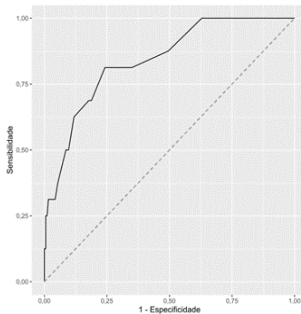
Fig. 1. ROC Curve
