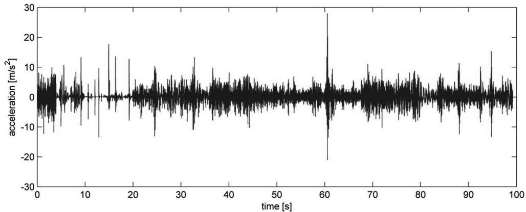
Fig. 4. Vibration profile of rms = 2,14m/s 2
