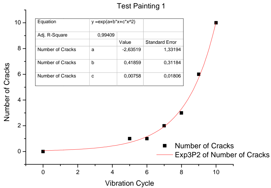
Fig. 7. Total number of cracks measured after each vibration cycle. The crack growth is exponential
