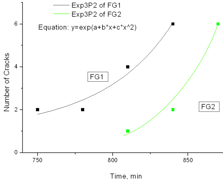
Fig. 10. Number of surface cracks of samples FG1 and FG2 measured in time, after each vibration cycle. The growth of crack number is clearly exponential
