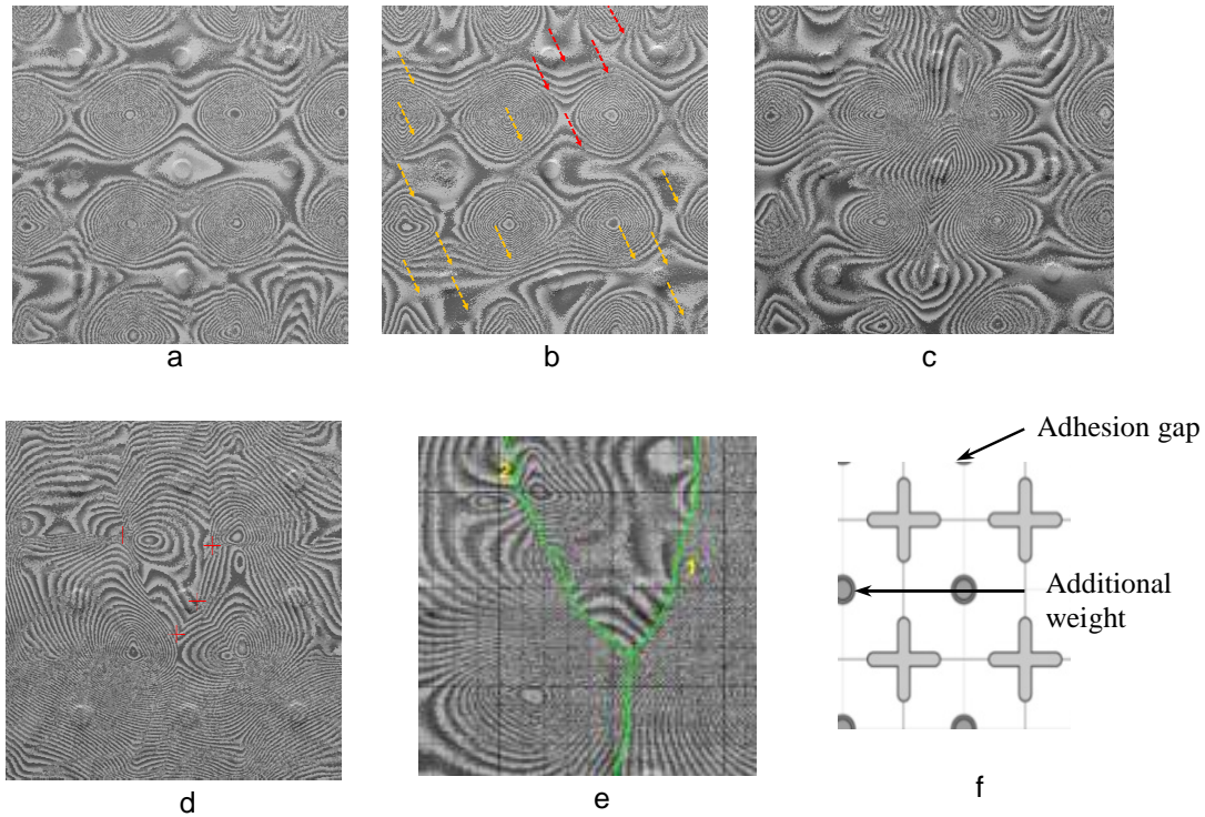
Fig. 9. Example of interferograms, a) reference interferogram -before vibration loading- of sample FG2 according to the sample construction shown in Fig. 3, b) after 1 st vibration cycle at t=30 min. Orange arrows show potential yet hidden cracks. Red arrow shows the first surface crack that appeared after 7 th vibration cycle at t=810 min, c) with red arrows indicating the full length of the crack, d) FG2 after 9 th vibration cycle and at t= 890 min, e) zoom-in surface crack map studied from interferograms of sample FG2 showing the first two surface cracks and f) zoom-in known defect map
