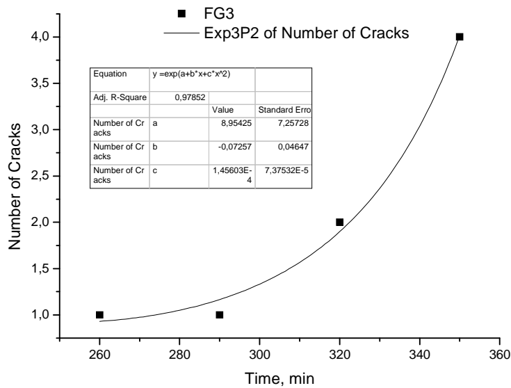
Fig. 11. Number of surface cracks of sample FG3 measured in time, after each vibration cycle. The growth of crack number is clearly exponential
