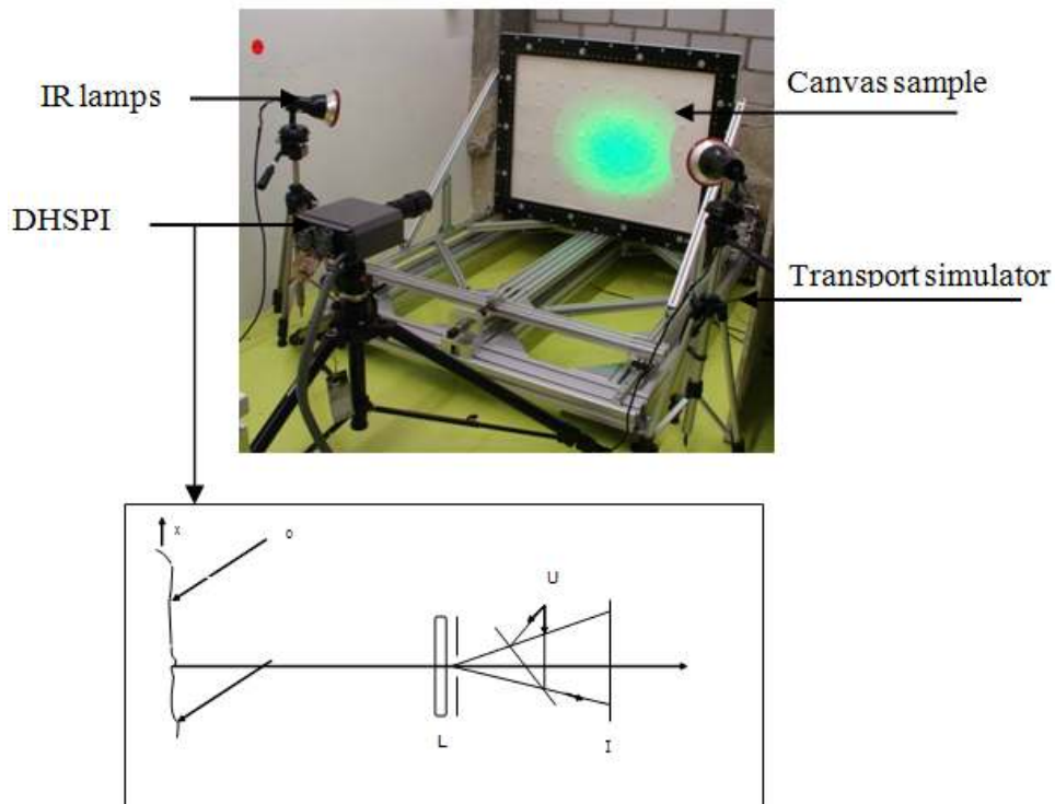
Fig. 1. Photograph of the DHSPI monitoring system and transport simulator set up with optical geometry to provide a holographic correlation interferometer with U inline reference beam sensitive to out of plane displacement of surface and object illumination beam O, L lens assembly and I the CCD position level
