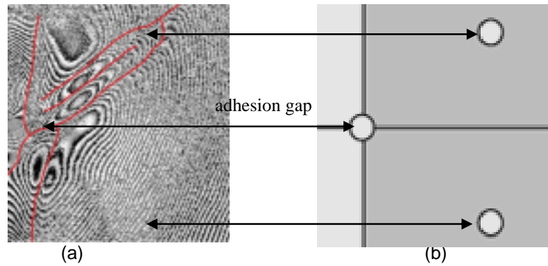
Fig. 6. Interferometric example of local crack map registered from interferograms after 10 th vibration cycle at t=100 min compared to known induced defect map, in a) crack map resulted from interferograms of sample TP1, propagation length marked in red, and b) the known defect map. Note detachment generation seen as circular fringes among cracks. Most defected fringes are developed in the area with the pre-existing defects are denser
