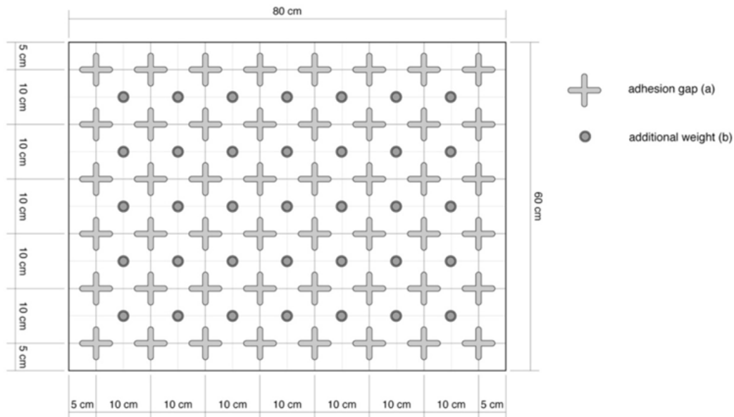
Fig. 3. Schematic of canvas sample with known structural defects on the sample
