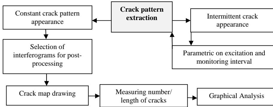
Fig. 5. Schematic representation of the experimental measuring methodology
