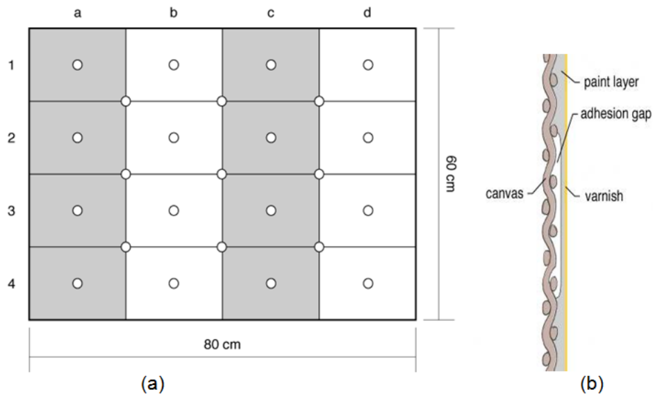
Fig. 2(a) Schematic of a sample, Circles indicate the location of weak spots, (b) Schematic of the construction of the sample
