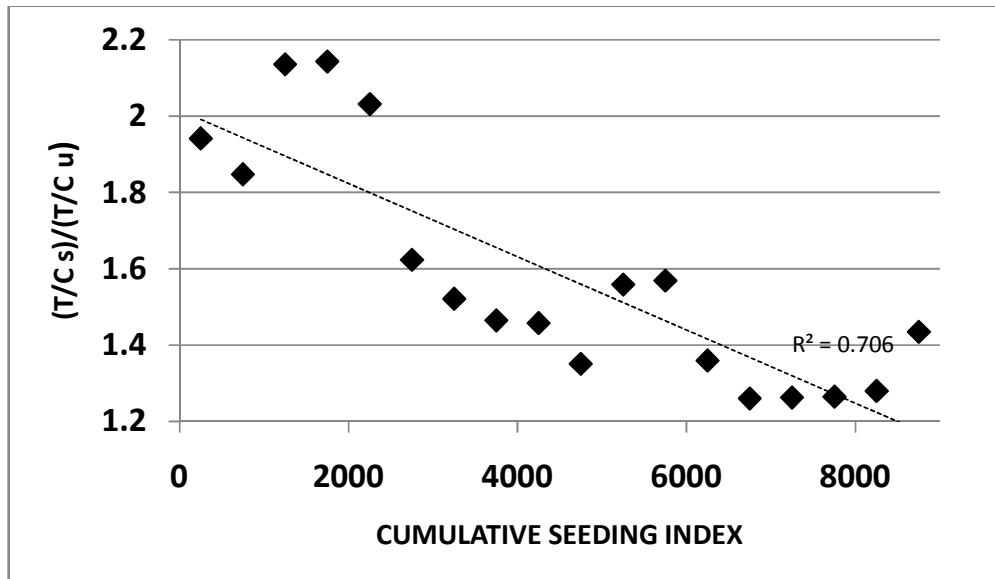
Fig. 4. Comparison of mean (T/C_{seeded}/T/C_{unseeded}) as a function of CSI at intervals of 500 for the Snowy Mountains experiment of 1955-1959
