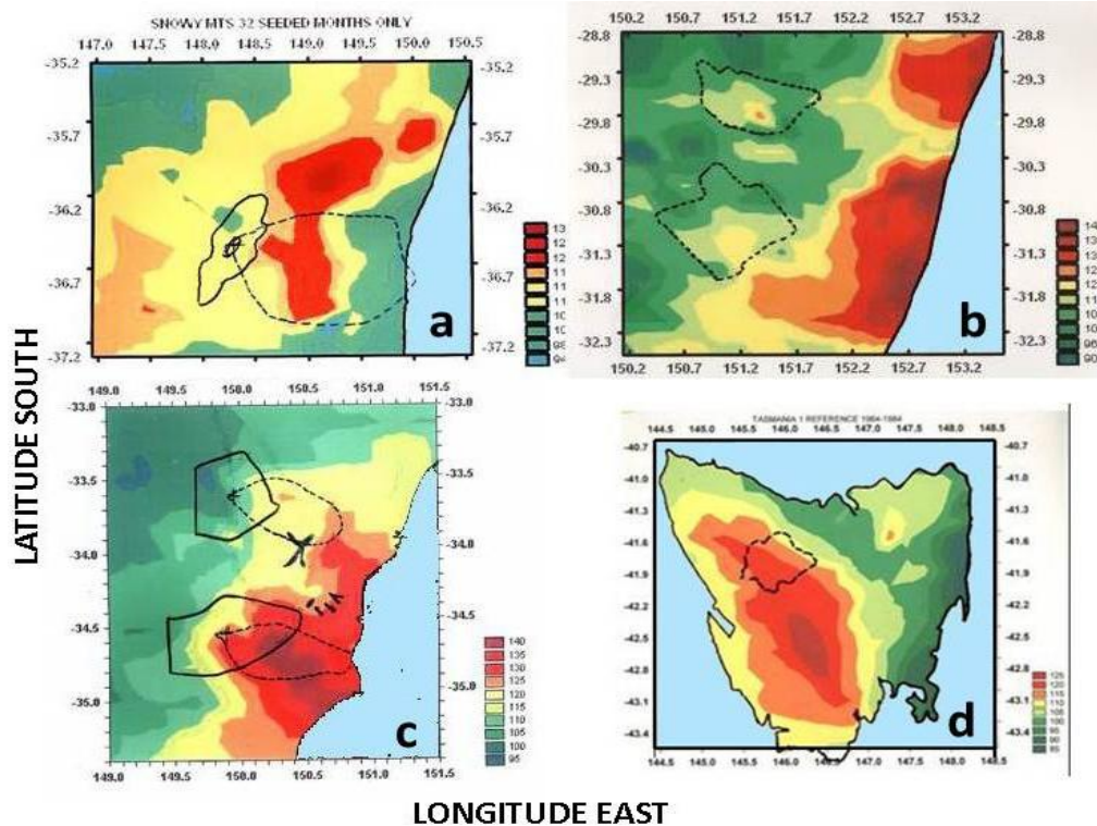
Fig. 7. Target areas of four early cloud seeding experiments shown by solid lines in a and c, dashed lines in b and d. The diagrams show contours of the ratio of mean rainfalls in seeded months to the means in corresponding months of seven unseeded years. The distribution of wind directions on seeded days are shown as dashed lines in a and c. Red areas have ratios >1.2
