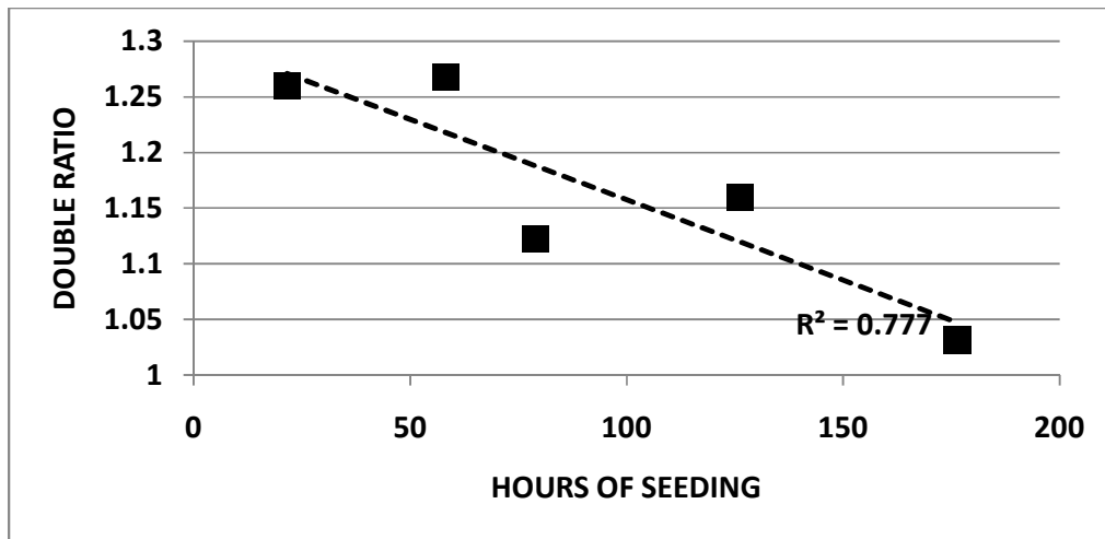
Fig. 3. In the snowy mountains experiment, E measured by the double ratio decreased substantially as the number of hours of seeding per year increased. E used period totals, not just seeded days
