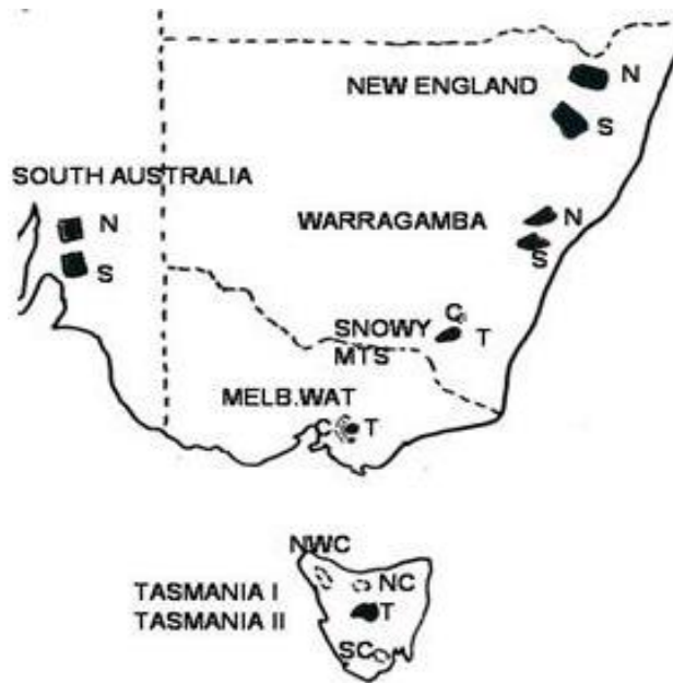
Fig. 1. Location of area cloud seeding experiments in south-east Australia, 1955-1992. Target areas are labelled T for single target experiments or N and S for crossover experiments, unseeded control areas are labelled C
