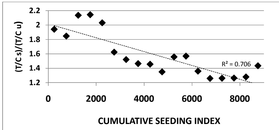
Fig. 5. Target/Northwest control precipitation on days suitable for seeding (ss), divided by the same ratio for days suitable for seeding but unseeded (su), compared with the cumulative seeding index. This measure of E refers to individual days only, not to period totals
