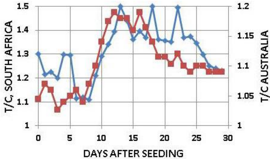
Fig. 6. Mean (Target/Control) on each day 1 to 30 following seeding divided by the mean T/C for the preceding 30 days. South African experiment: blue, Australian experiments: red. Note the different scales
