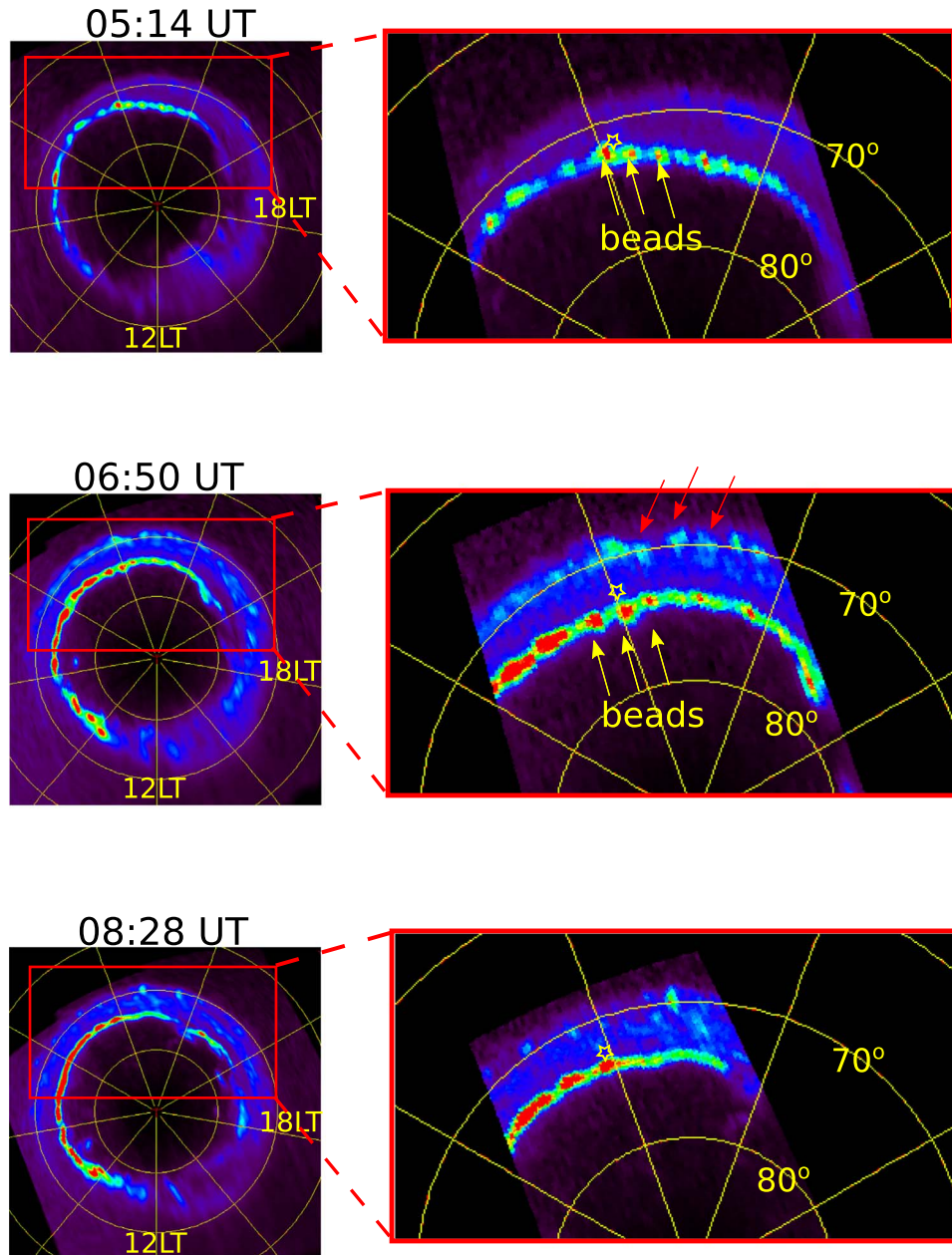
Figure 1. Sequence of polar projections of Saturn’s southern aurora obtained with the FUV channel of UVIS on board Cassini during the Cassini proximal orbits. The first image starts at 0514 UT and the last one at 0828 UT on DOY 232, 2017. Noon is to the bottom and dusk is to the right. The grid shows latitudes at intervals of 10^\circ and meridians every 30^\circ . Each panel of the right column displays one of the subimages used to reconstruct the corresponding complete image on the left. The yellow arrows indicate some of the auroral beads on the main emission and the red ones those on the low latitude emission. The yellow star points out to the magnetically mapped location of the Cassini spacecraft at the time of the observation.
