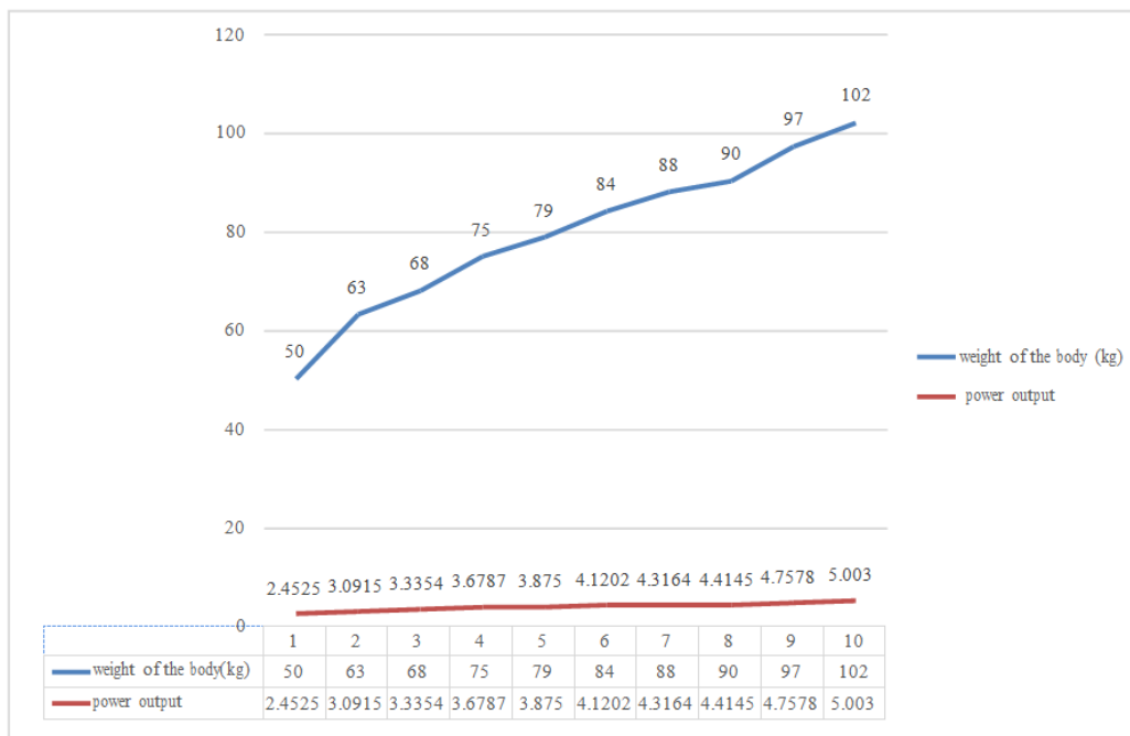
Fig. 3. Graph of weight induced against power generated
