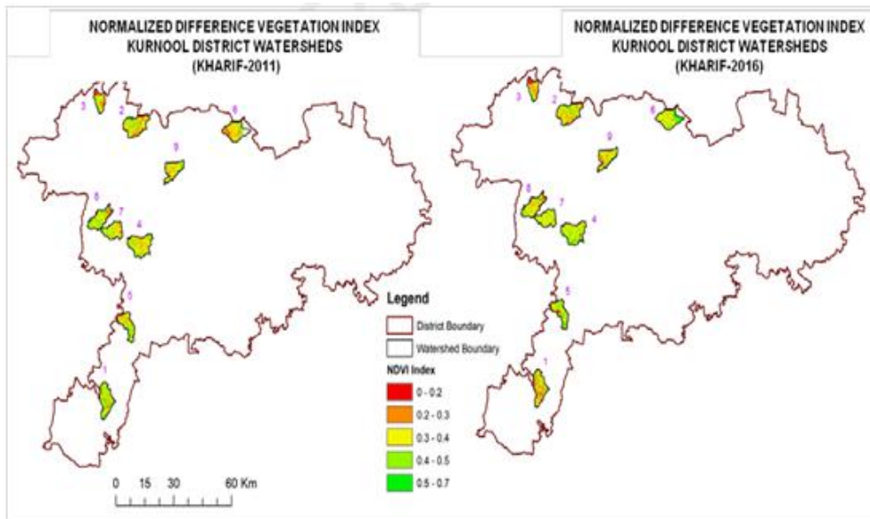
Fig. 4. Normalized difference vegetative index comparison for 2011 and 2016
