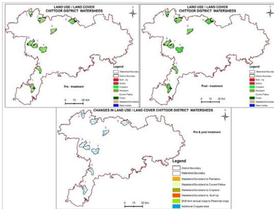
Fig. 5. Land use land cover maps comparison
