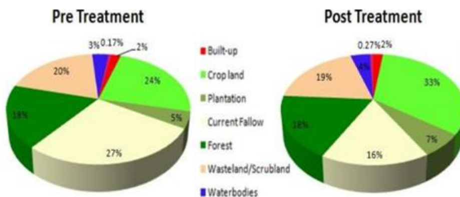
Fig. 6. Land use / Land cover distribution
