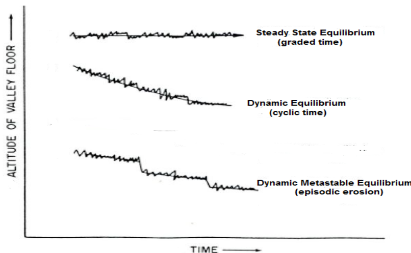
Fig. 1. Dynamic Metastable Equilibrium Source: Schumm [18], Modified by the Authors, (2021)
