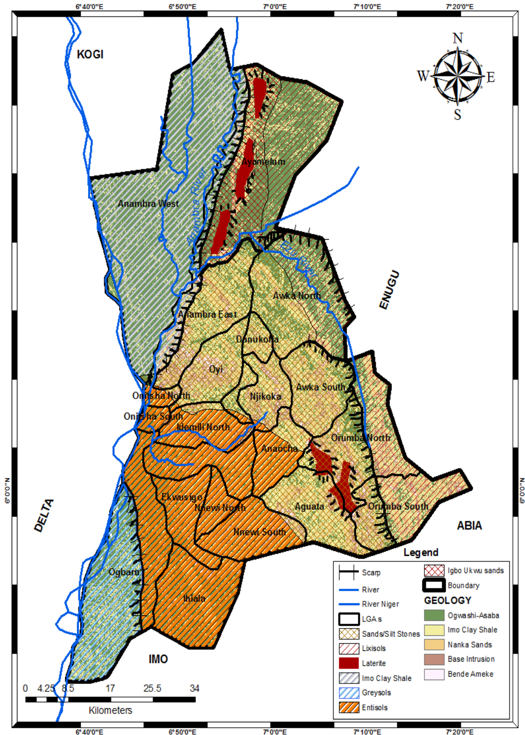
Fig. 4. Geology and Soils of Anambra State
