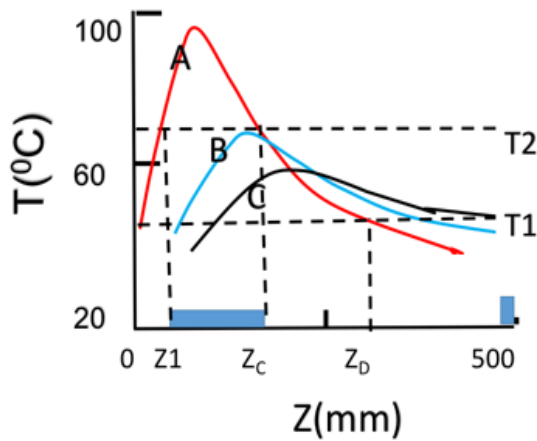
Fig. 7. Calculated temperature spatial profiles (at irradiation time t=250\text{ ms} ) for various A=(30,60,90)\text{ cm}^{-1} for Curve-C, -B, -A, and a fixed I_0=3\text{ W/cm}^2
