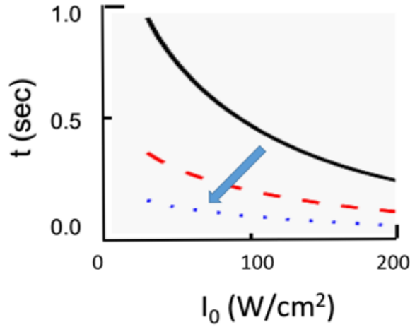
Fig. 5. The calculated irradiation time needed ( t ) to reach a surface temperature of 60\text{ }^{\circ}\text{C} , for various A=(30,40,90)\text{ cm}^{-1} , for curves from top to low, for an irradiation time of 0.5 s
