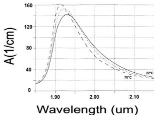
Fig. 9. Water absorption spectra at different temperatures (solid: 22°C, dotted: 49°C, dashed: 70°C), after Ref. [11]
