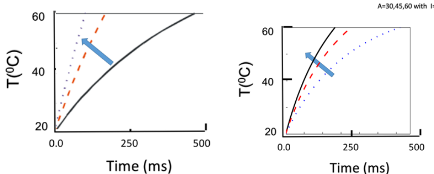
Fig. 1. Calculated surface temperature profiles T(z=0) (Left) for the effects of laser intensity, I_0=(50,100,200) \text{ W/cm}^2 , for curves right to left, for a fixed A=60 \text{ cm}^{-1} . (Right) temperature profiles for a fixed I_0=100 \text{ W/cm}^2 , but for various A=(30,45,60) \text{ cm}^{-1} , for curves right to left Fig. 1. Calculated surface temperature profiles T(z=0) (Left) for the effects of laser intensity, I_0=(50,100,200) \text{ W/cm}^2 , for a fixed A=60 \text{ cm}^{-1} . (Right) temperature profiles for a fixed I_0=200 \text{ W/cm}^2 , but for various A=(30,45,60) \text{ cm}^{-1}
