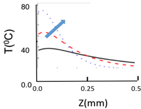
Fig. 3. Calculated temperature spatial profiles T(z) at a given laser irradiation time ( t=500 \text{ ms} ) for A=(15, 30, 60) \text{ cm}^{-1} , for curves low to top with a fixed I_0=200 \text{ W/cm}^2 , and heat transport coefficient range of G= 0.5 \text{ WC/cm}^2
