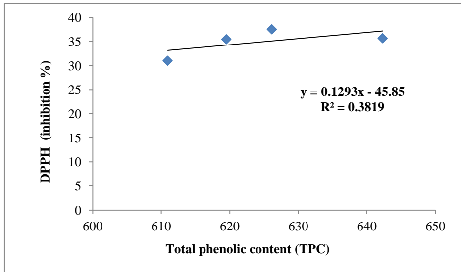
Fig. 2. Linear correlation between the antioxidant activity data from DPPH assays and the total phenolic content (TPC) of Chinese essential oil
