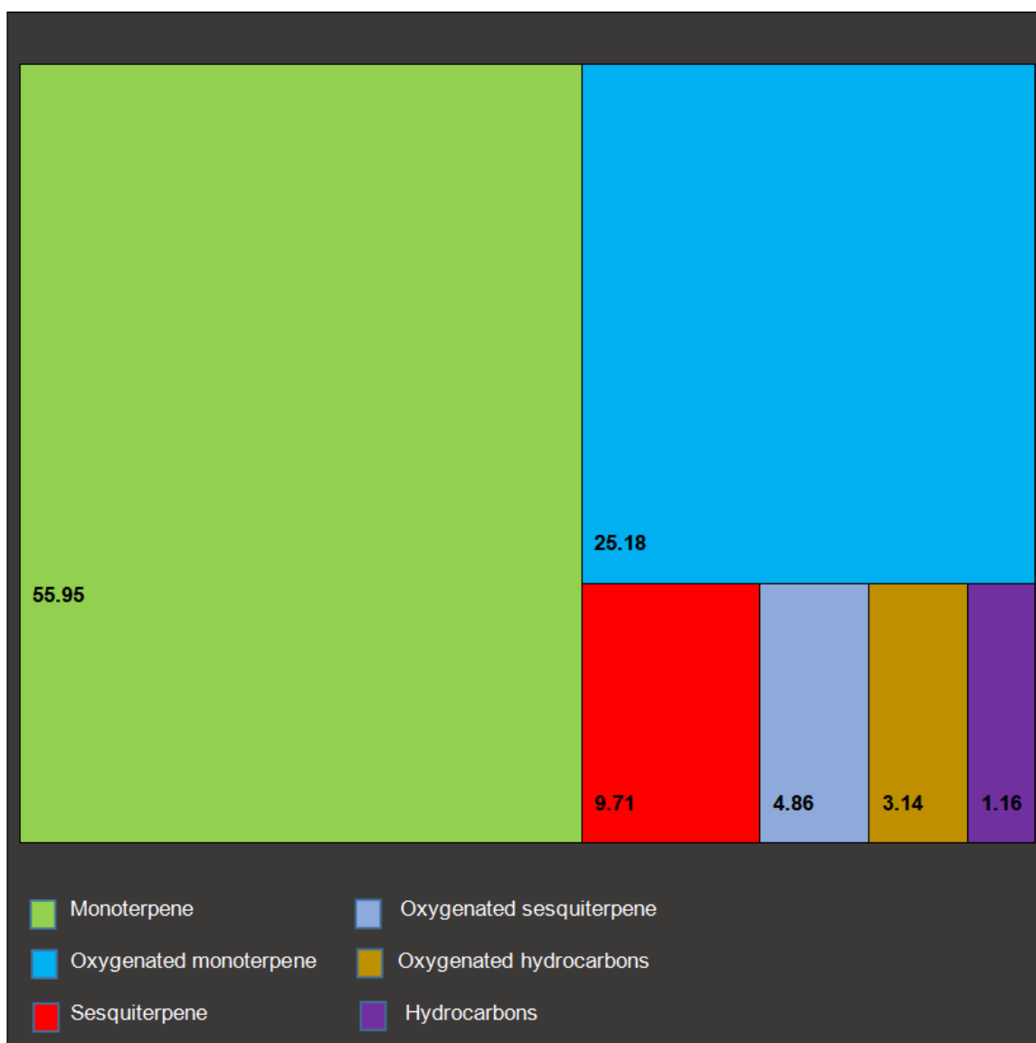
Fig. 1. Major classification of lemon essential oil components identified
