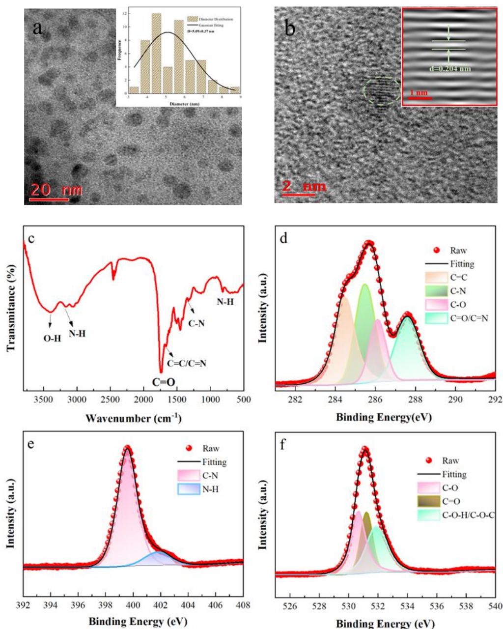
Fig. 1. (a) TEM image of the N-CDs. (b) HRTEM image of the N-CDs. (c) FT-IR spectra of the N-CDs. (d) C1s ,(e) N1s and (f) O1s high resolution spectra of the N-CDs
