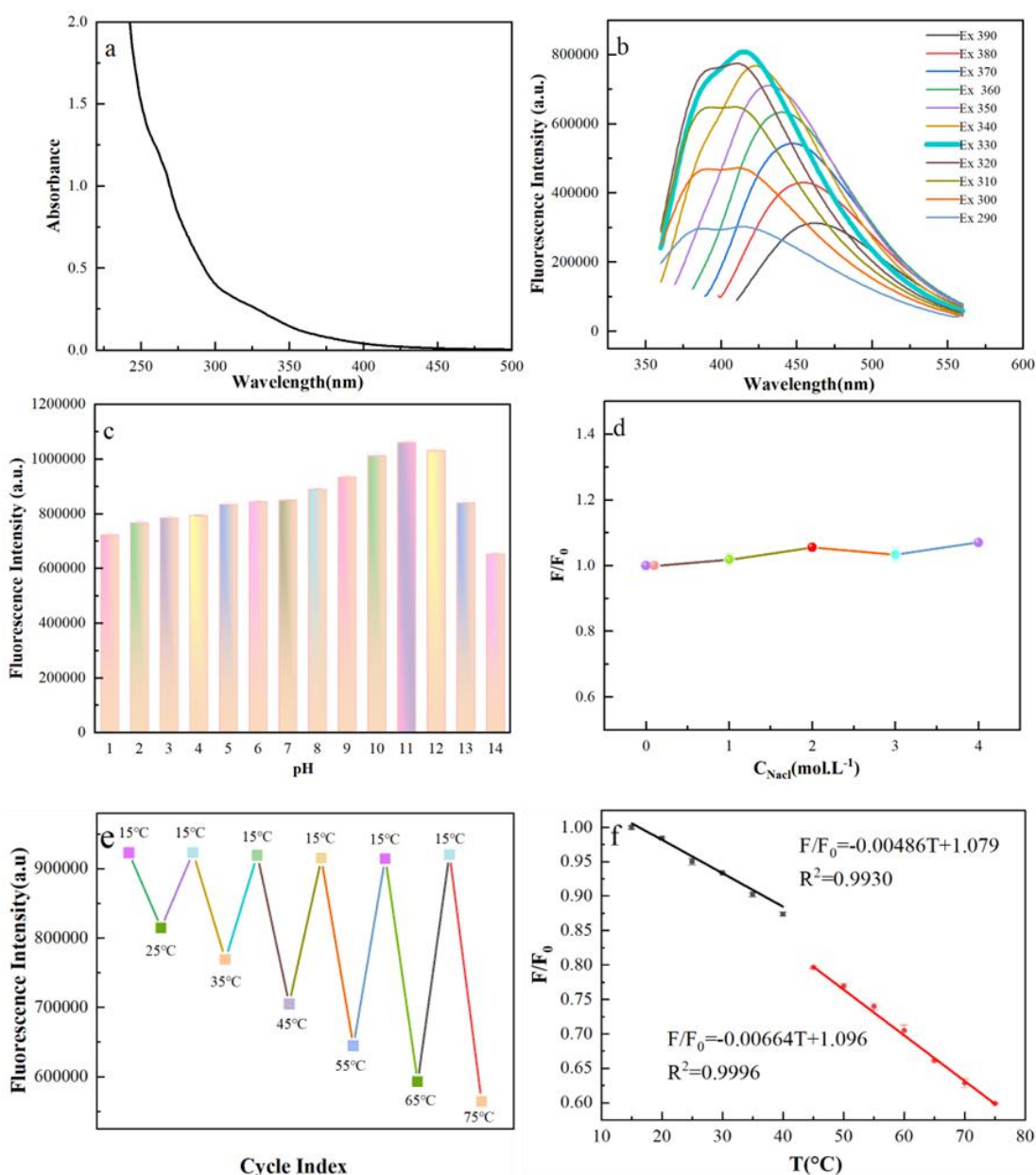
Fig. 2. (a) UV-vis absorption spectra of the N-CDs. (b) Fluorescence emission spectra of N-CDs. (c) Effect of pH on the fluorescence intensity of N-CDs. (d) Effect of NaCl on the fluorescence intensity of N-CDs. (e) Cyclic testing of temperature response with N-CDs. (f) F/F_0 versus temperature plots of N-CDs with temperature range of 15 °C -75 °C
