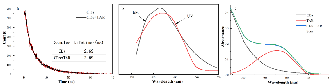
Fig. 5. (a) Fluorescence decay curve of N-CDs in the absence and presence of TAR. (b) spectra overlap between fluorescence emission spectrum of N-CDs and absorption spectrum of TAR. (c) absorption spectra of N-CDs, TAR, N-CDs-TAR mixtures and the sum value of absorbance of N-CDs and TAR
