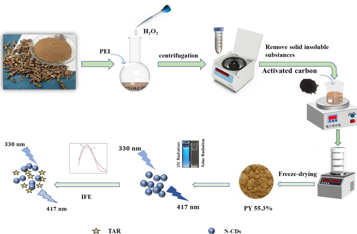
Scheme 1. A. schematic diagram of the preparation strategy of N-CDs and the sensing principles for TAR
