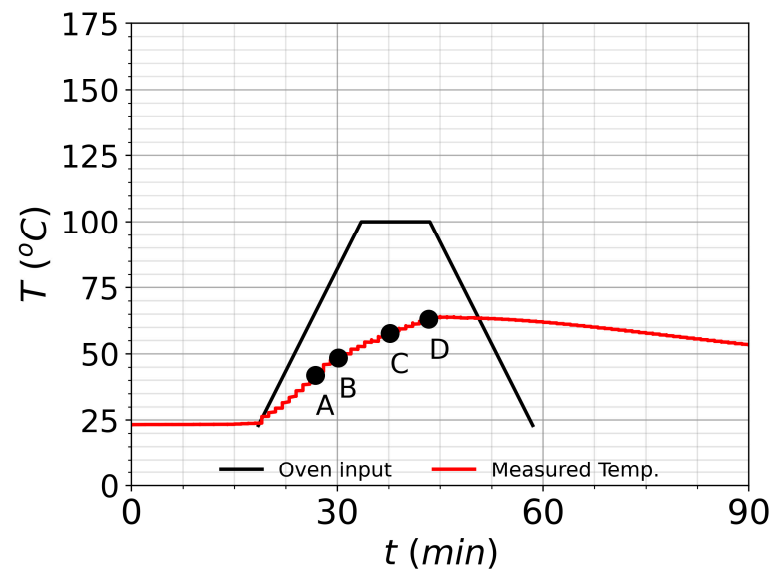
Figure 11. Heating cycle for aluminum alloy plate.
