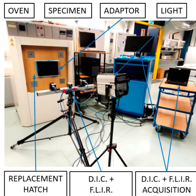
Figure 10. Test setup.
