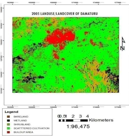
Fig. 3.3 2005 LULC of Damaturu
