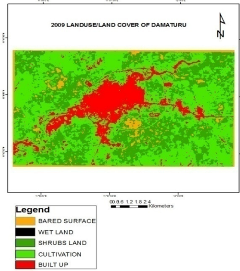
Fig. 3.4 2009 LULC of Damaturu
