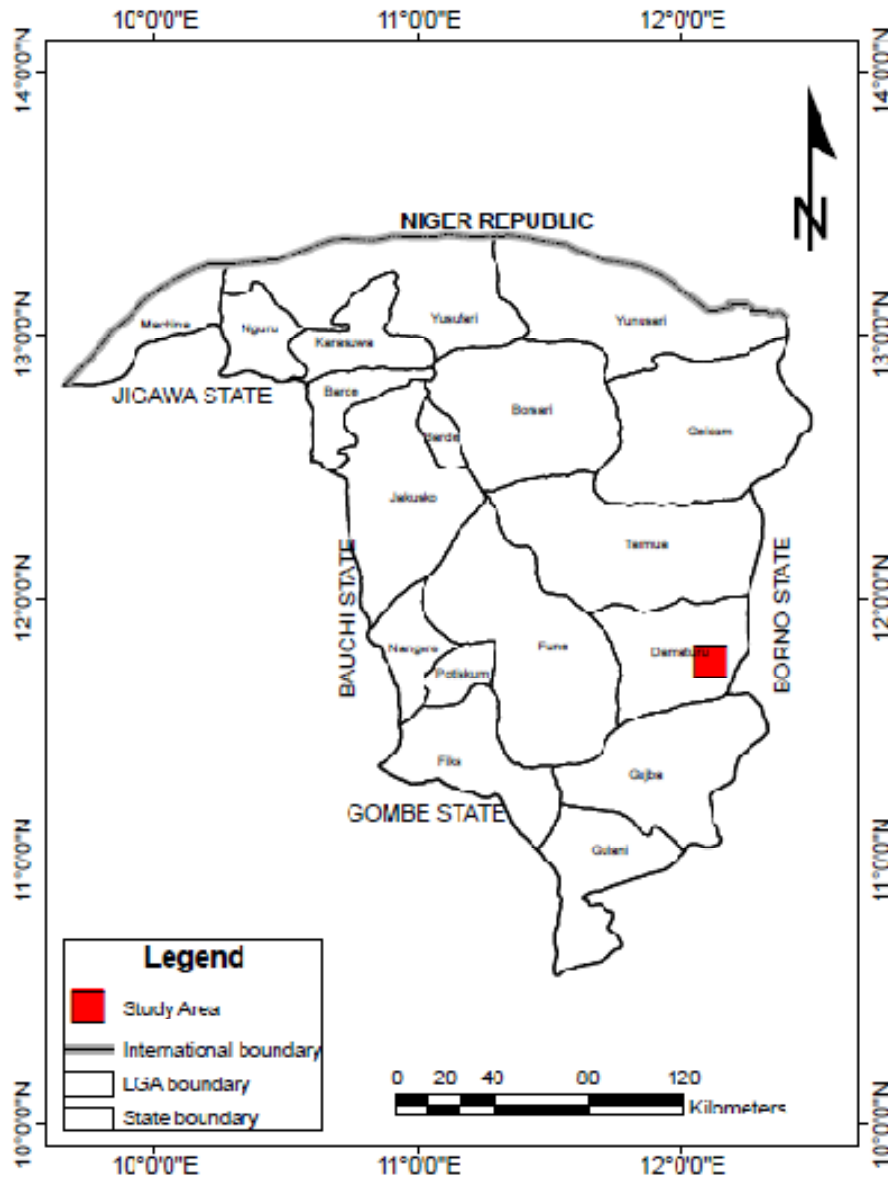
Fig. 1. Yobe State Showing Damaturu Source: Yobe State Ministry of Lands and Survey
