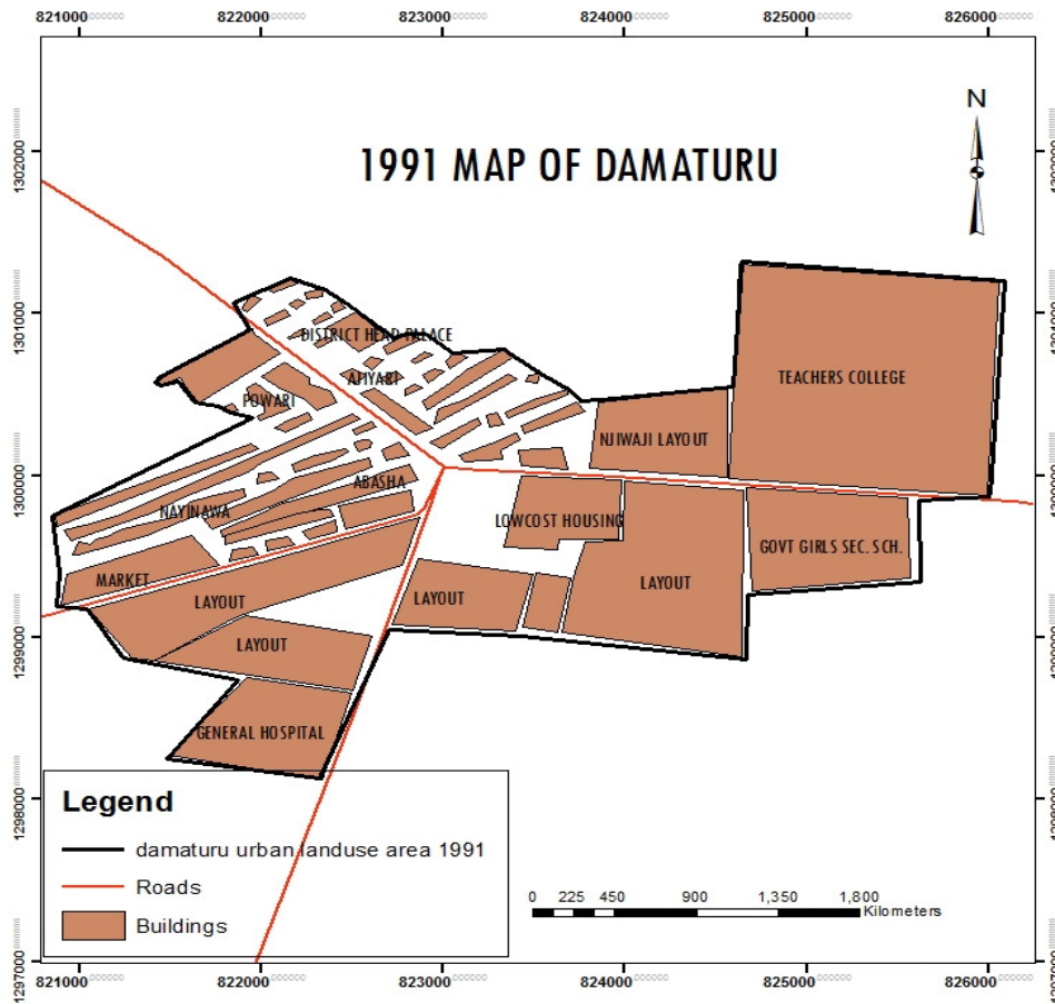
Fig. 2. Damaturu before state creation
