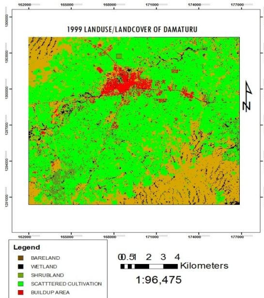
Fig. 3.2 1999 LULC of Damaturu
