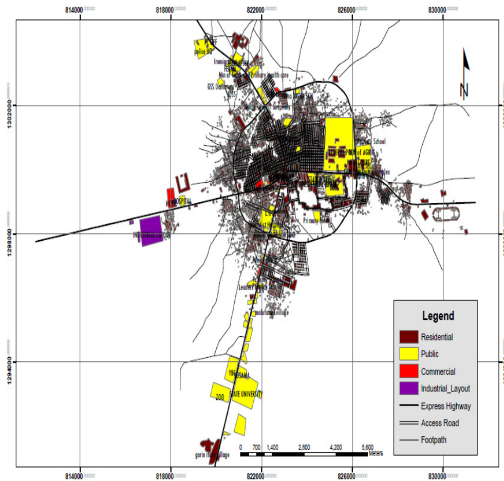
Fig. 4. Damaturu urban landuse Source: Google earth image
