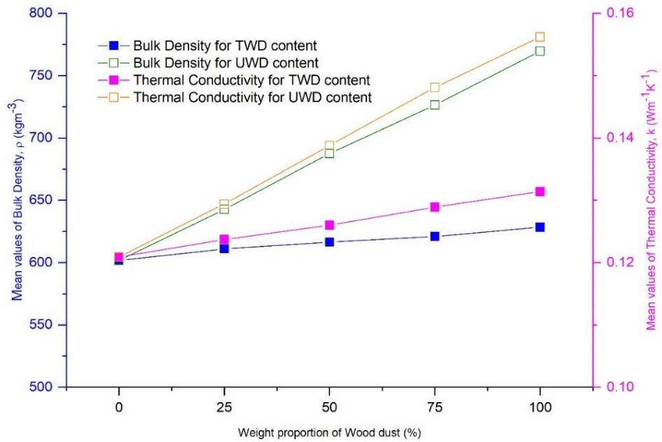
Fig. 2. Variations of bulk density and thermal conductivity of the samples with proportion of the wood dust
