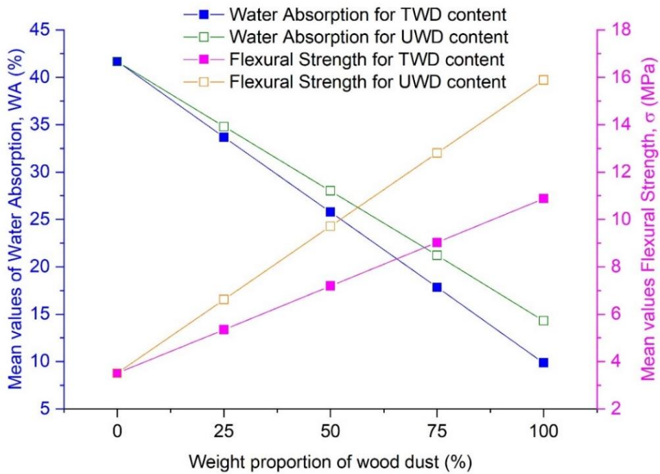
Fig. 3. Variations of water absorption and flexural strength of the samples with proportion of the wood dust
