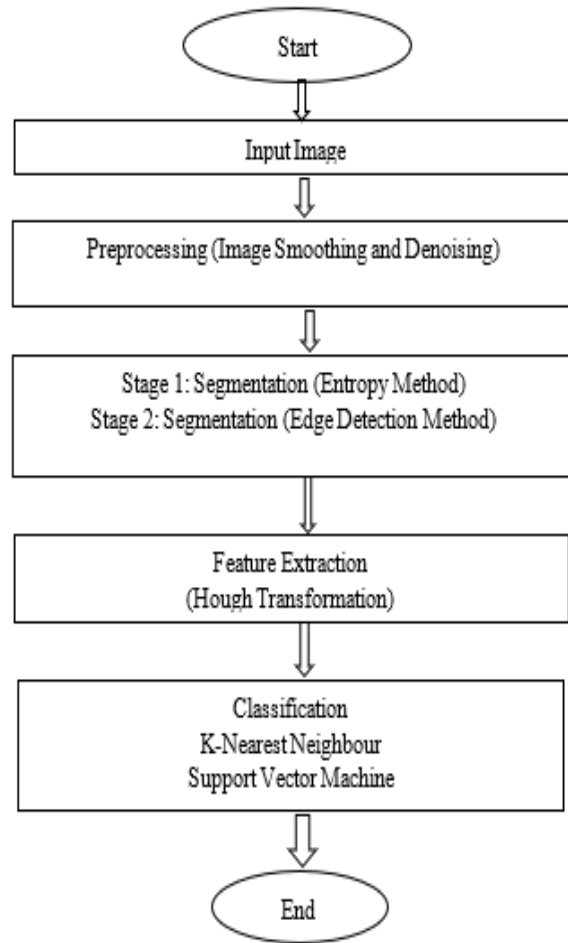
Fig. 1. Categorization of fracture bones stages
